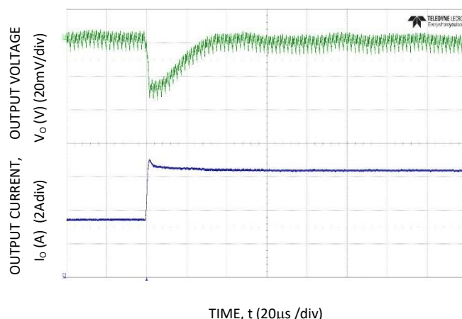
Figure 16. Transient Response to Dynamic Load Change from 50% to 100% at 12Vin, C_{out}=3x47\mu F+1x330\mu F , C_{Tune}=3.9nF , R_{Tune}=300\Omega
