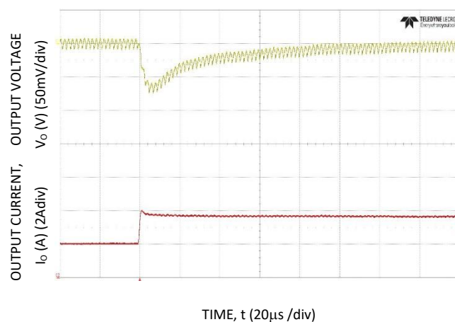
Figure 28. Transient Response to Dynamic Load Change from 50% to 100% at 12Vin, C_{out}=3 \times 47\mu\text{F} , C_{Tune}=470\text{pF} , R_{Tune}=300
