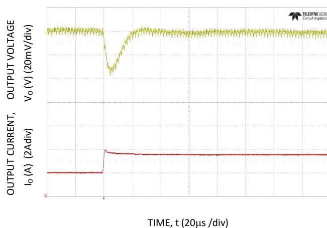
Figure 16. Transient Response to Dynamic Load Change from 50% to 100% at 12Vin, C_{out}=5x47\mu F , C_{Tune}=4.7nF , R_{Tune}=300
