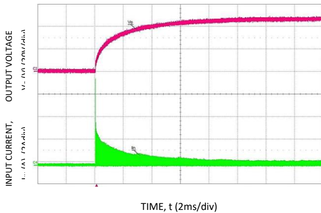
Figure 1. Inrush Current
