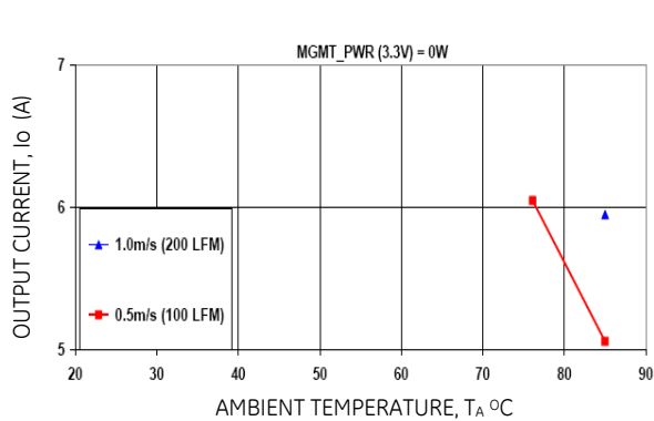
Figure 13-1. PIM300F Derating Output Current versus Local Ambient Temperature and Airflow ( V_{in} = -48Vdc ; MGMT\_PWR, 3.3V = 0W )
