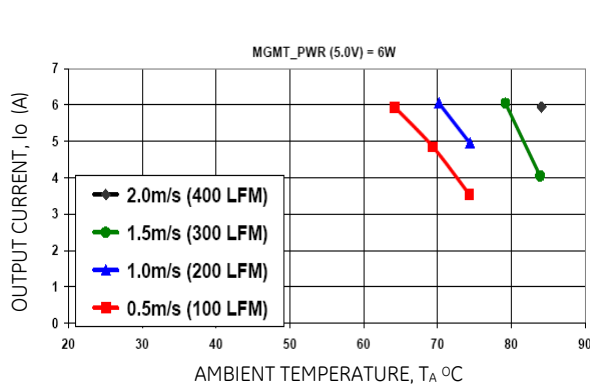
Figure 14-3. PIM300A Derating Output Current versus Local Ambient Temperature and Airflow ( V_{in} = -48Vdc ; MGMT_PWR, 5.0V = 6W)
