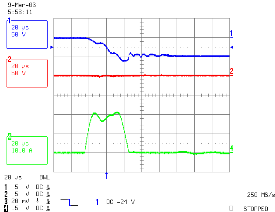
Figure 2. Inrush Current
