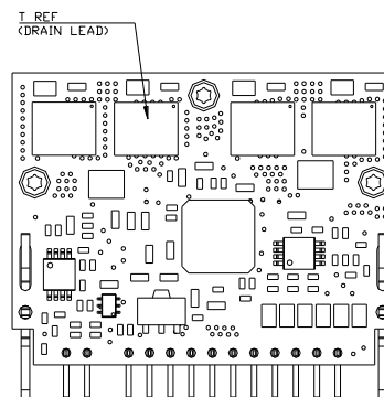
Figure 46. Temperature measurement location T_{ref} .
