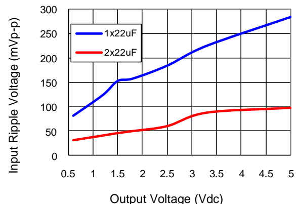
Figure 40. Input ripple voltage for various output voltages with 1x22 μF or 2x22 μF ceramic capacitors at the input (40A load). Input voltage is 12V.
