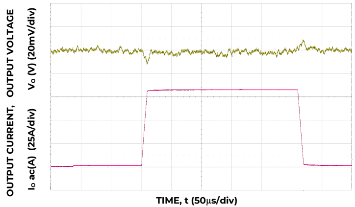
Figure 22. Trans. Resp. to 100A/μs Load Change from 25% to 75% at 12V_{IN} , C_o=4 \times 0.047\mu\text{F} + 4 \times 0.1\mu\text{F} + 15 \times 22\mu\text{F} + 73 \times 47\mu\text{F} + 6 \times 470\mu\text{F} polymer.
