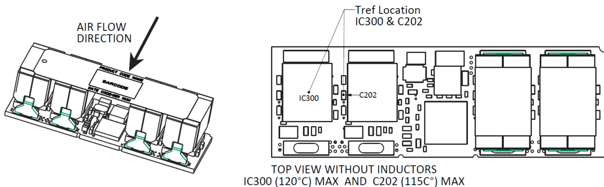
Figure 29. Preferred airflow direction and the location of the thermal reference points
