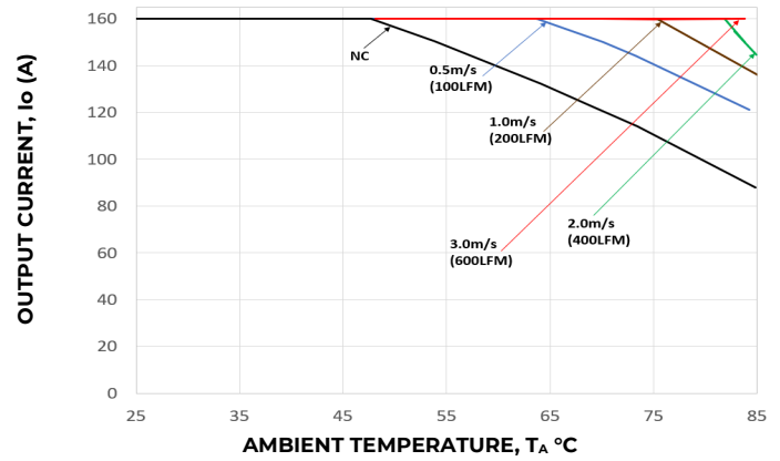
Figure 20. Derating Output Current versus Ambient Temperature
