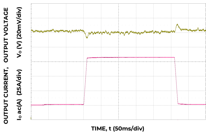
Figure 10. Trans. Resp. to 100A/μs Load Change from 25% to 75% at 12V in , C_o = 4 \times 0.047\mu\text{F} + 4 \times 0.1\mu\text{F} + 15 \times 22\mu\text{F} + 73 \times 47\mu\text{F} + 6 \times 470\mu\text{F} polymer.
