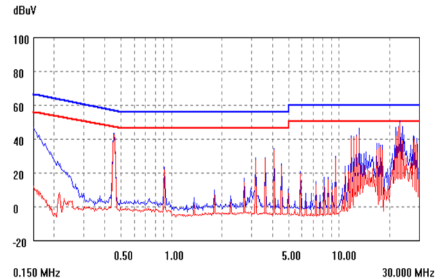
Figure 17. EMC signature using above filter, KSTW015A0.
