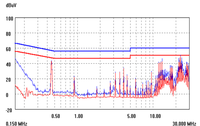
Figure 17. EMC signature using above filter, KSTW010A0.
