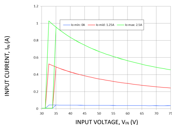
Figure 2. Converter Input Current versus Input Voltage.
