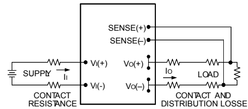
Figure 17. Circuit Configuration for remote sense.
