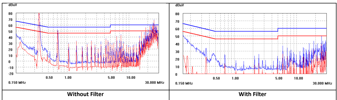
Figure 22. EMC Considerations
