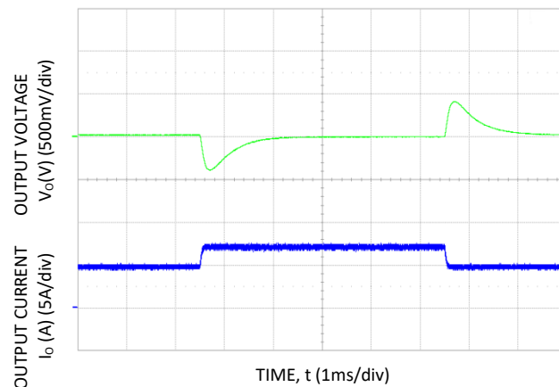
Figure 6. Dynamic Load Change Transient Response from 50% to 75% to 50% of Full Load at Room Temperature and 48V in ; 0.1A/μs, C_{o,ext} = 440\mu F .
