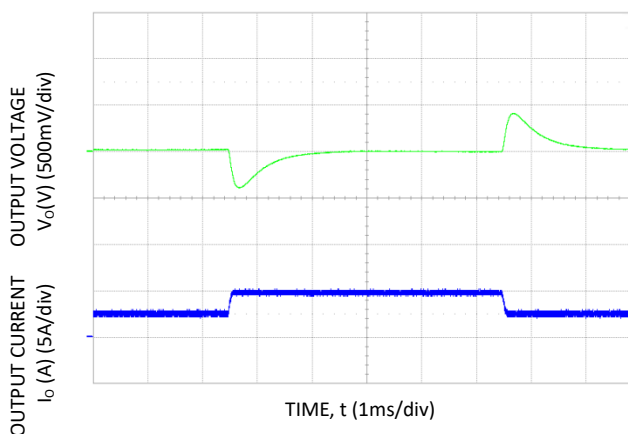
Figure 3. Dynamic Load Change Transient Response from 25% to 50% to 25% of Full Load at Room Temperature and 48V in ; 0.1A/μs, C_{o,ext} = 440\mu F .
