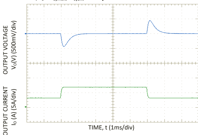
Figure 3. Dynamic Load Change Transient Response from 25% to 50% to 25% of Full Load at Room Temperature and 48 Vin; 0.1A/μS, C_{o,ext} = 440\mu F .
