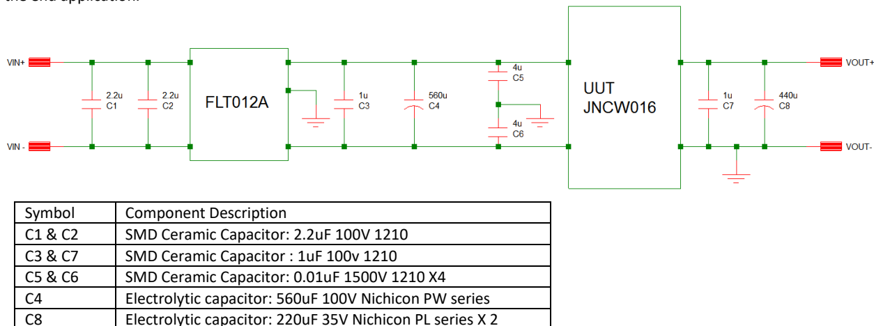
Figure 23. EMC Filter
