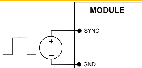
Figure 4. External source connections to synchronize switching frequency of the module.
