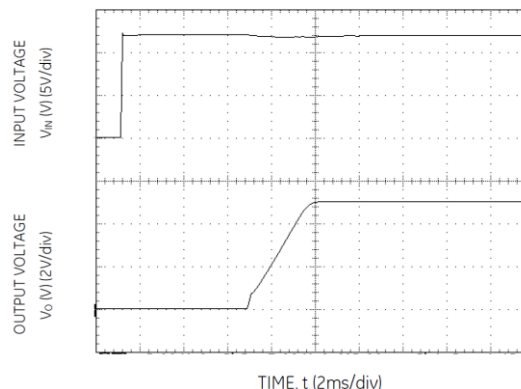
Figure 2. Typical Start-up using Input Voltage ( V_{in}=12\text{V} , V_{out} = V_{out, \text{max}} , I_{out} = I_{out, \text{max}} )
