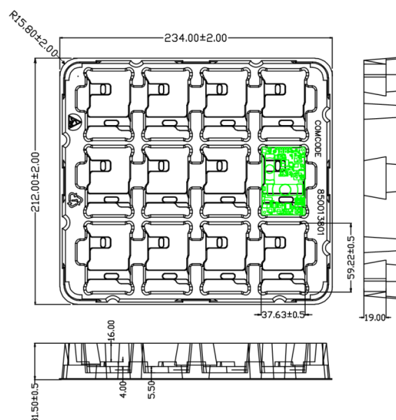
Figure 26. QSD(V)W050 Packaging Tray (Base Plate Module Tray)
