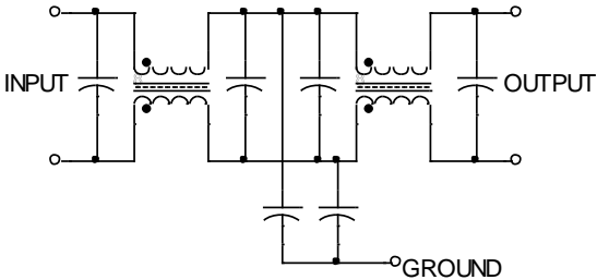
Figure 4. Internal Schematic
