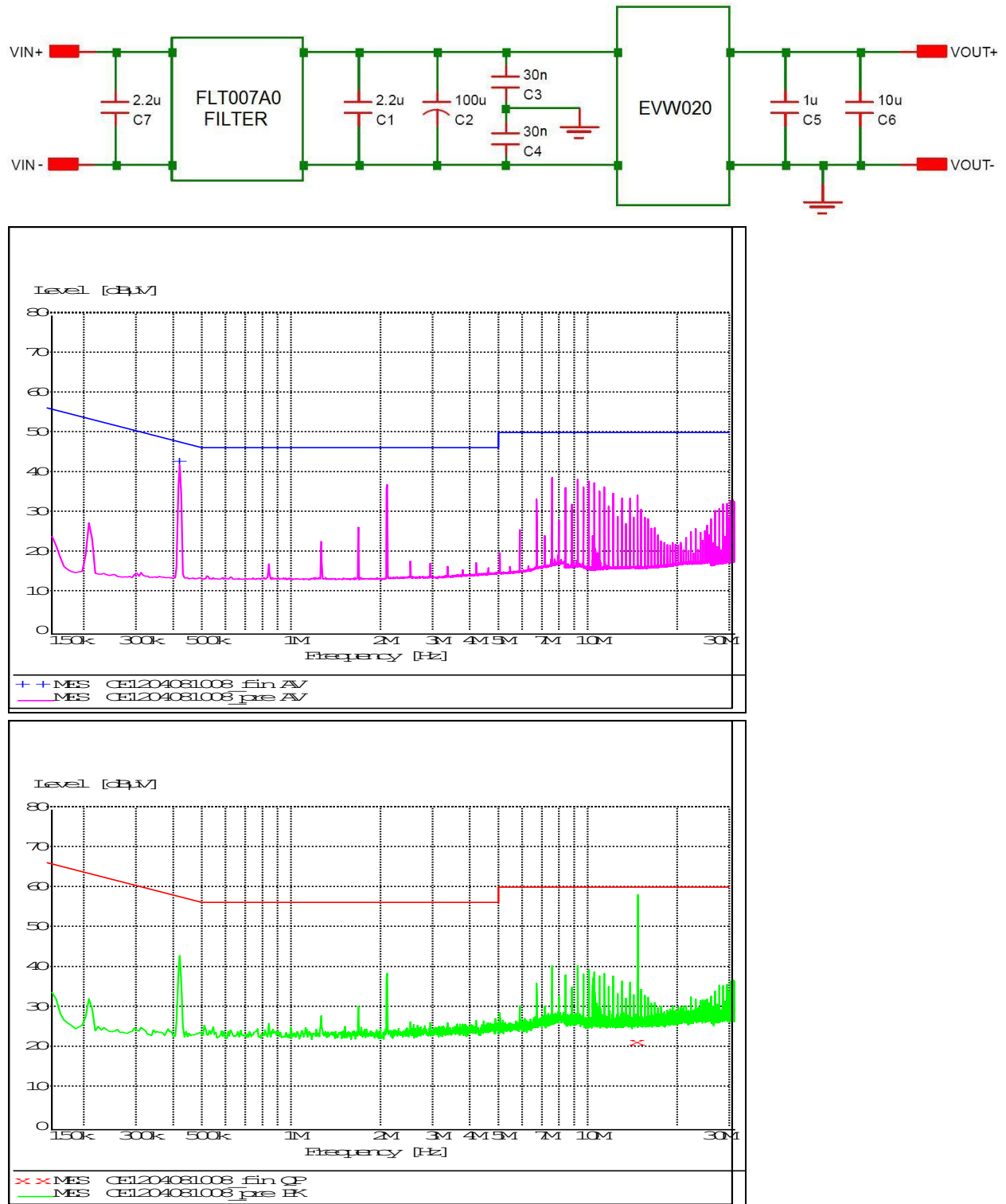
Figure 25. EMC Considerations
