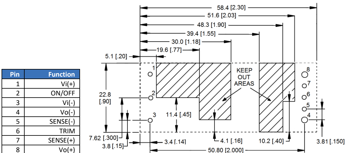
SMT Recommended Pad Layout (Component Side View)
