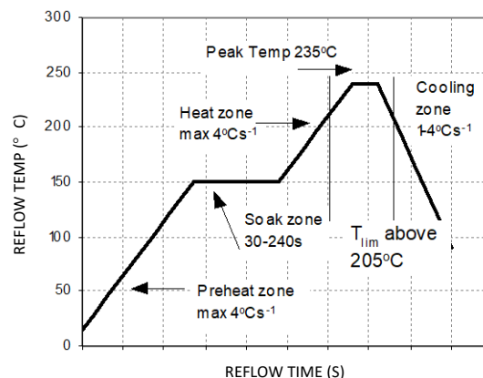
Figure 16. Reflow Profile for Tin/Lead (Sn/Pb) process.
