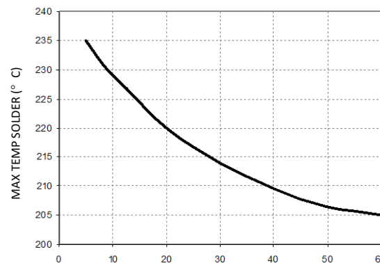
Figure 17. Time Limit Curve Above 205°C for Tin/Lead (Sn/Pb) process
