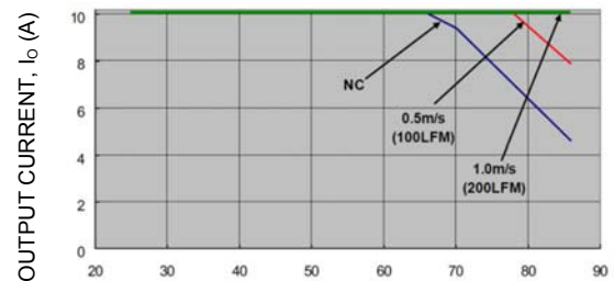
Figure 15. Output Current Derating for the Open Frame Module; Airflow in the Transverse Direction from Vout(+) to Vout(-); Vin = 48V.
