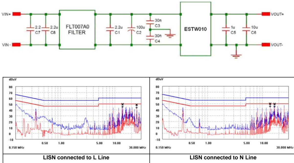
Figure 25. EMC Considerations
