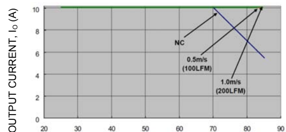
Figure 17. Output Current Derating for the Open Frame Module with Heatplate and 0.25” Heatsink; Airflow in the Transverse Direction from Vout(+) to Vout(-); Vin = 48V.
