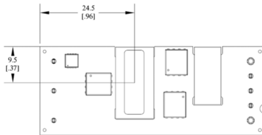
Figure 21. Pick and Place Location.
