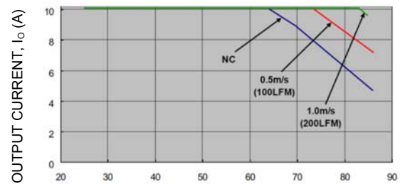
Figure 15. Output Current Derating for the Open Frame Module; Airflow in the Transverse Direction from Vout(+) to Vout(-); Vin = 48V.
