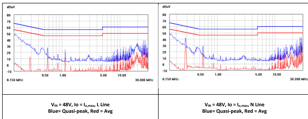
Figure 25. EMC Considerations.
