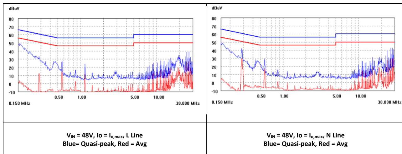
Figure 25. EMC Considerations.
