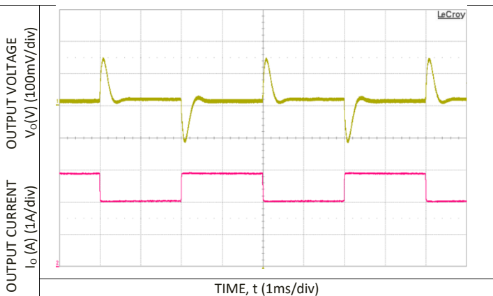
Figure 6. Dynamic Load Change Transient Response from 50 % to 75% to 50% of Full Load at Room Temperature and 48 Vin; 0.1A/uS, C_{o,ext} = 220\mu\text{F} .
