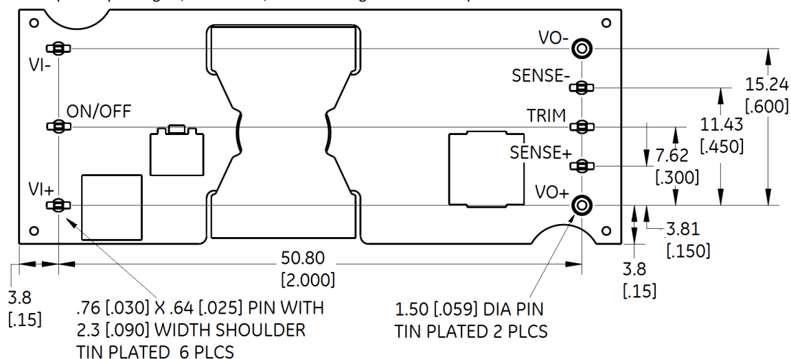
BOTTOM VIEW
