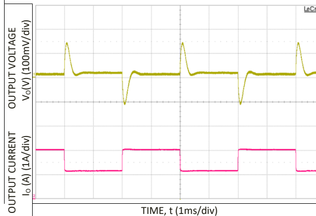
Figure 3. Dynamic Load Change Transient Response from 25% to 50% to 25% of Full Load at Room Temperature and 48 Vin; 0.1A/uS, C_{o,ext} = 220\mu\text{F} .
