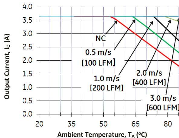
Figure 21. Derating Output Current vs. local Ambient temperature and Airflow, open frame or No baseplate, V_{in} = 48V, airflow from V_i(-) to V_i(+) .
