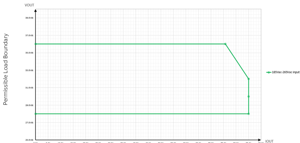
CC2725AC34TZL Output Current Curve
