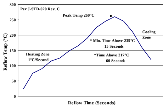
Figure 27. Recommended linear reflow profile using Sn/Ag/Cu solder.
