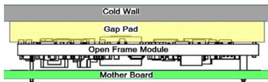
Figure 20. Cold Wall Mounting
