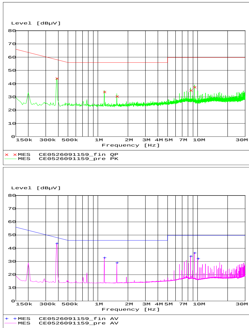
Figure 28. EMC Considerations
