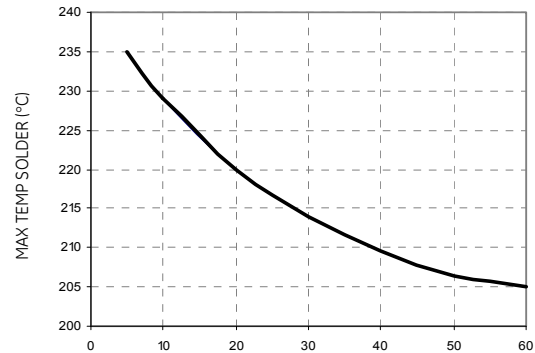
Figure 26. Time Limit Curve Above 205°C for Tin/Lead (Sn/Pb) process
