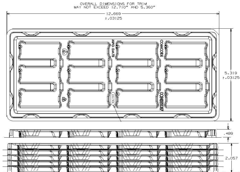
Figure 29. Surface Mount Packaging Tray
