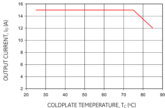
Figure 21. Derated Output Current versus Cold Wall Temperature with local ambient temperature around module at 85°C; Vin=48V.
