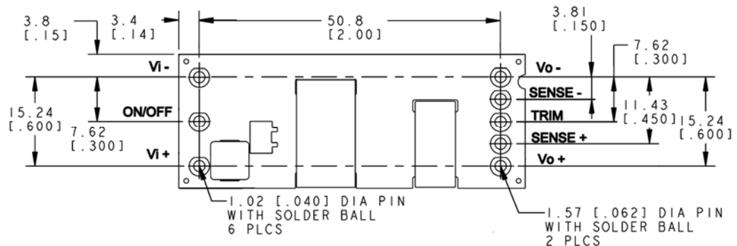
Bottom View
