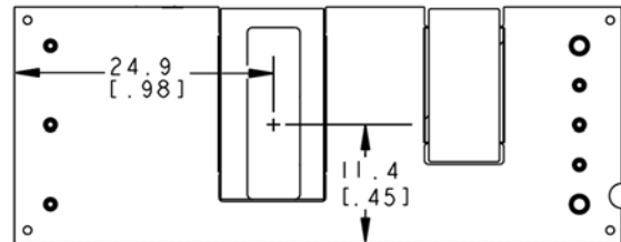
Figure 23. Pick and Place Location.
