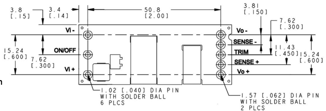
Bottom View
