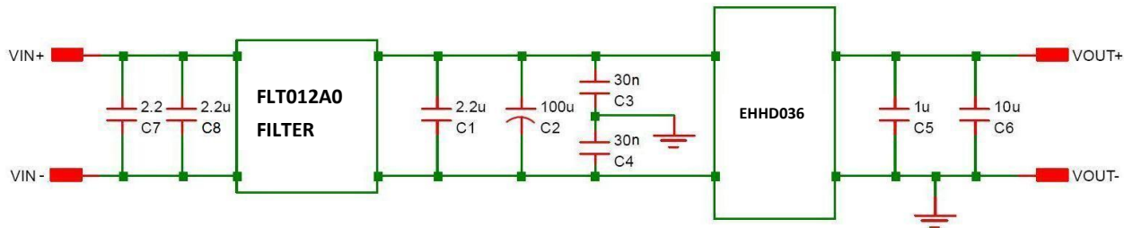
Figure 27. EMC Considerations
