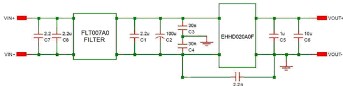
Figure 28. EMC Considerations
