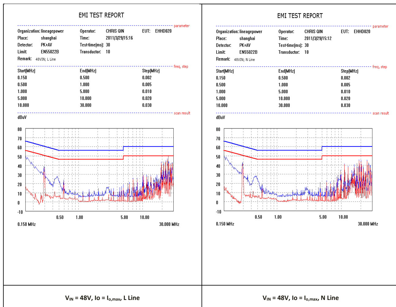
Figure 28. EMC Considerations
