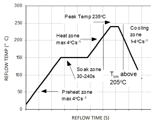
Figure 25. Reflow Profile for Tin/Lead (Sn/Pb) process.
