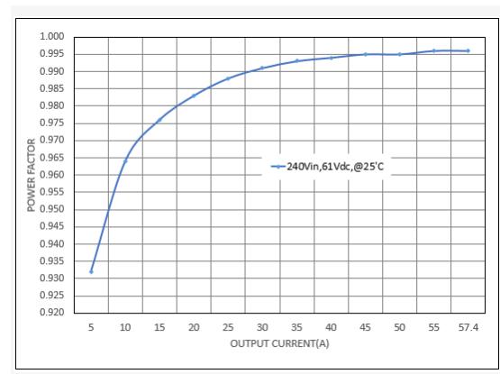
Figure 2. Power Factor versus Output Current
