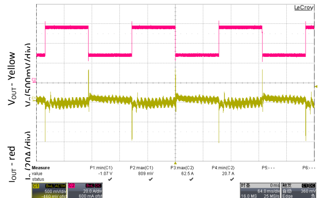
Figure 8. Transient response 65V DC load step 10 – 60%, Slew rate: 1A/μs, V IN = 230V AC
