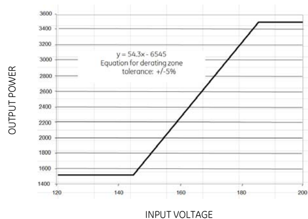
Figure 18. Output power derating below V_{IN} of 185VAC
