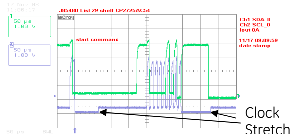
Example waveforms showing clock stretching.
