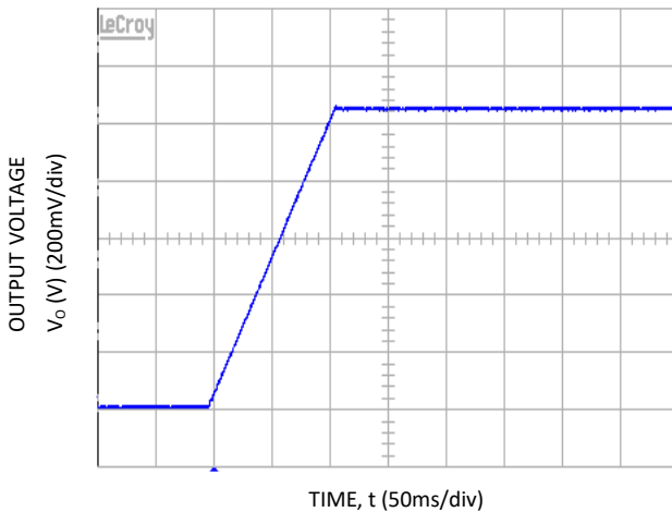
Figure 9. 54V DC soft start, no-load & full load, V_{\text{IN}}=185\text{V}_{\text{AC}} - I 2 C mode.
