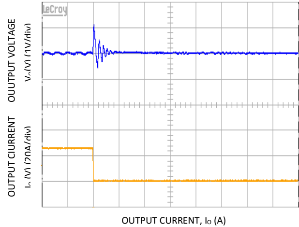
Figure 8. Transient response 54V DC load step 27.2 – 2.5A, V_{\text{IN}} = 185\text{V}_{\text{AC}} .
