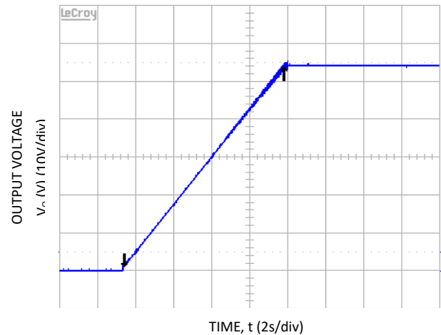
Figure 10. 54V DC soft start, full load, V_{\text{IN}} = 185\text{V}_{\text{AC}} - RS485 mode.
