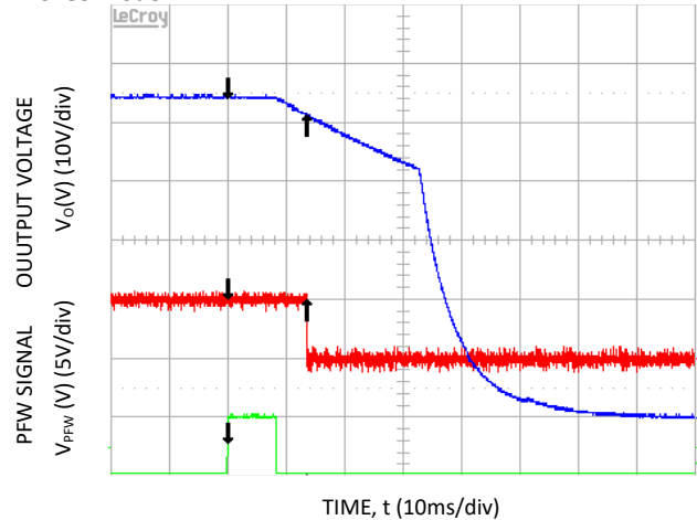
Figure 12. PFW alarmed 19.6ms prior to V_o < 40\text{V} , output load: 38A, V_{\text{IN}} = 185\text{V}_{\text{AC}} .
