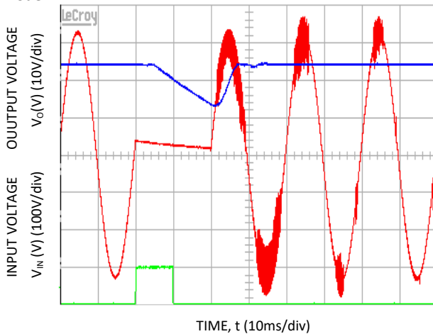
Figure 11. Ride through missing 1 cycle, full load, V_{\text{IN}} = 230\text{V}_{\text{AC}} .
