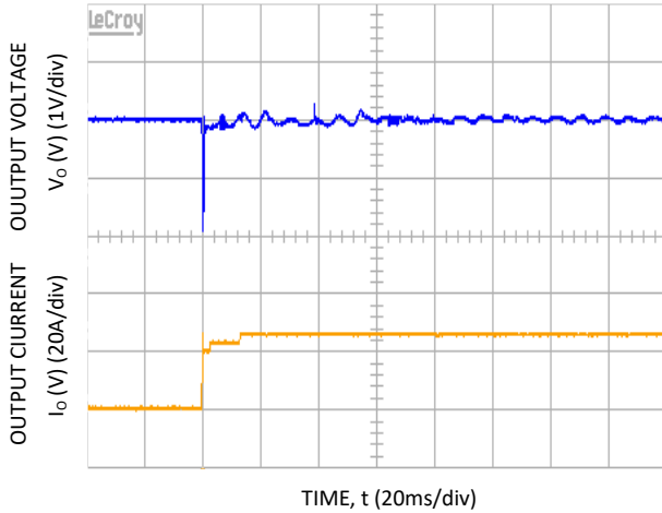
Figure 7. Transient response 54V DC load step 2.5 – 27.2A, V_{\text{IN}} = 185\text{V}_{\text{AC}} .
