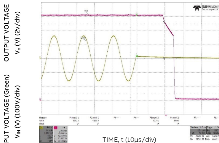
Figure 7. Typical Hold-up ( V_{IN} = 115V , 100% Load)
