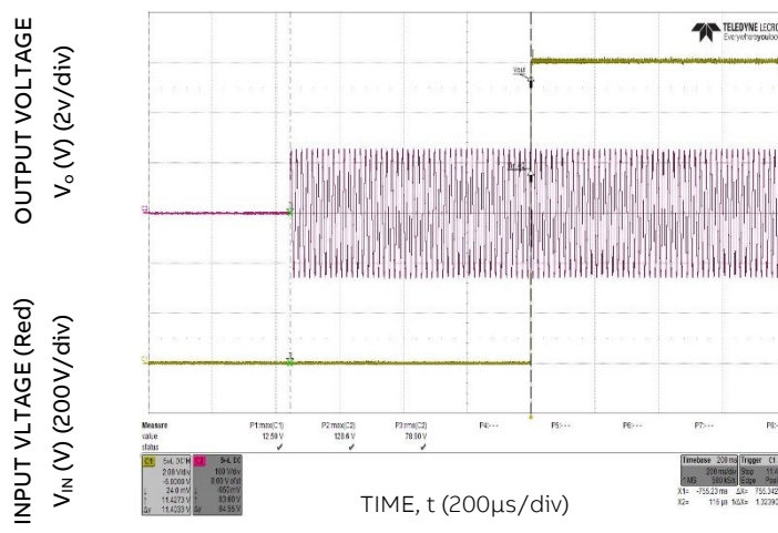
Figure 6: Typical Start-up ( V_{IN} = 230\text{Vac} , Full Load)
