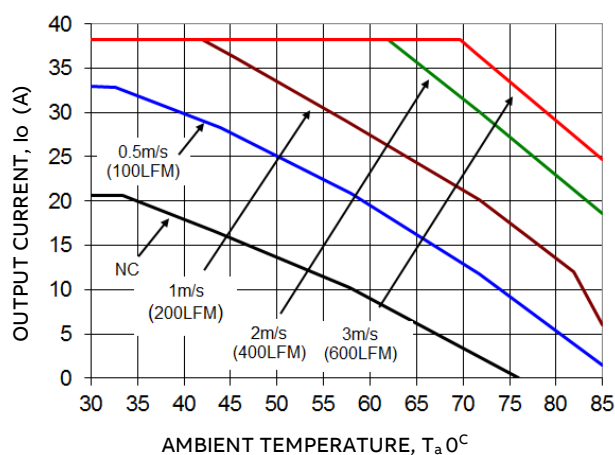
Figure 2: Power. Data shown for model CLP0412FPXXXZ03A, 115VAC in. At 230VAC in derating is the same or better. Standby output is loaded at 0.25A. For derating at other input voltages and other models, consult the GE Technical representative.
