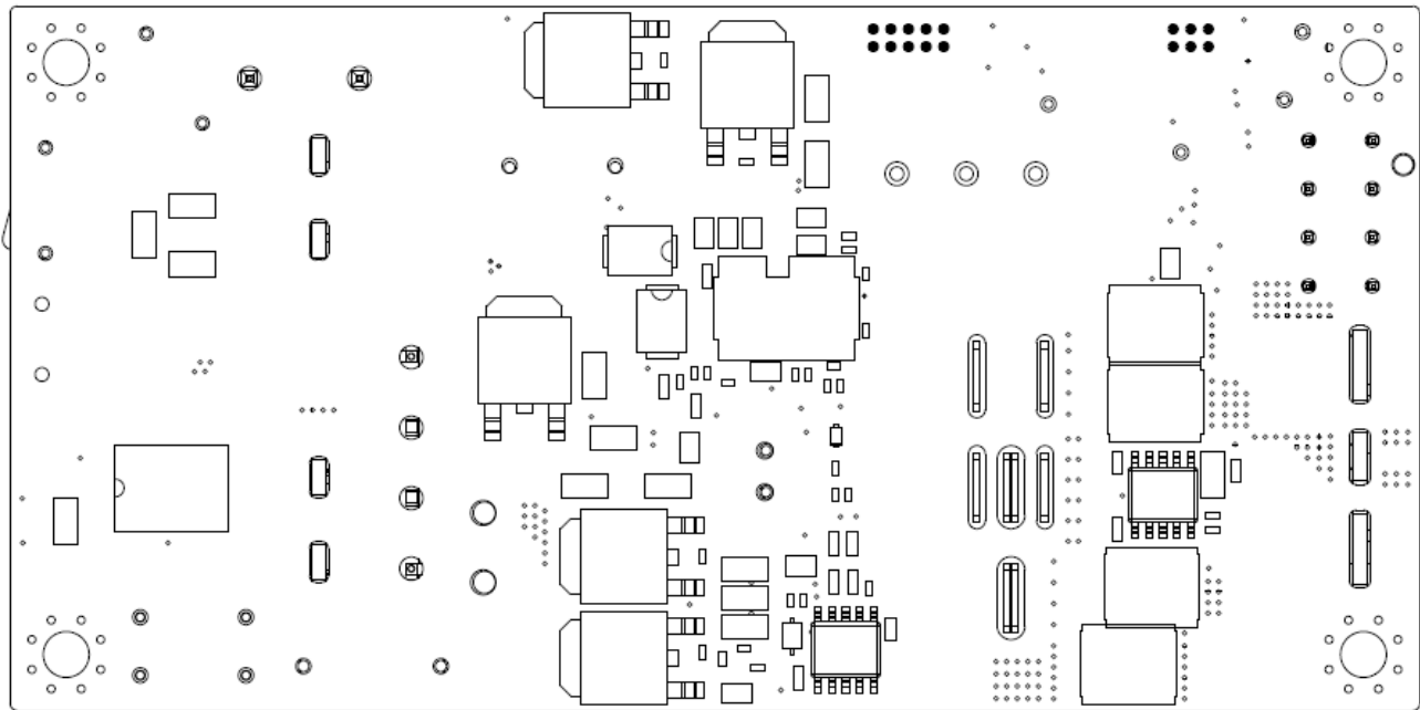
BOTTOM VIEW
