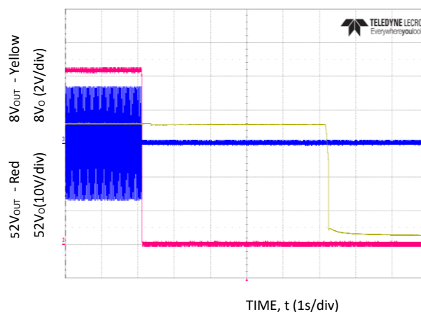
Figure 14. Turn-OFF at full load V_{IN} = 230V_{AC} .
