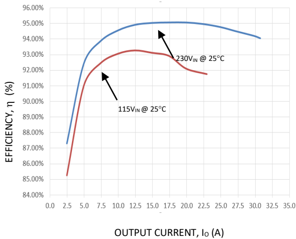
Figure 1. Rectifier Efficiency versus Output Current.
