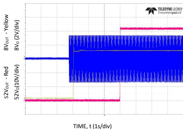
Figure 13. Turn-ON at full load V_{IN} = 230V_{AC}
