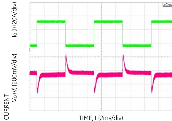
Figure 7. 12V transient response for 10 to 60% step load, V_{in} = -48V_{DC} , slew rate 1A/\mu s .
