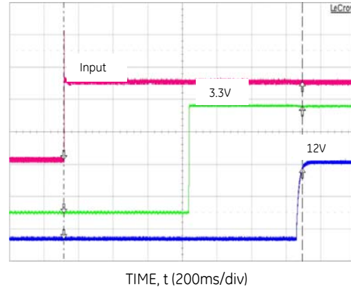
Figure 2. Input start up ( V_{in} = -48V_{DC} , full load).
