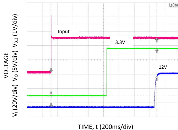
Figure 2. Input start up ( V_{in} : -48V_{DC} , full load).
