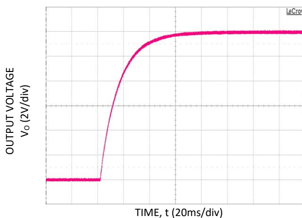
Figure 4. 12V start-up with 16,000 \mu f external capacitance ( V_{in} : -48V_{DC} , full load)
