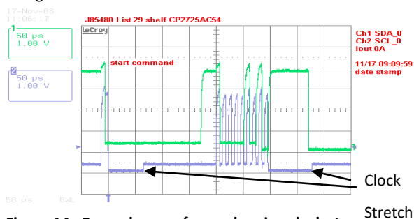
Figure 14. Example waveforms showing clock stretch
