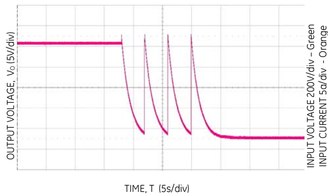
Figure 3. Overvoltage shutdown
