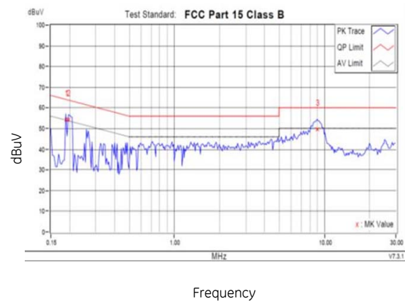
Figure 12. Conducted Emissions
