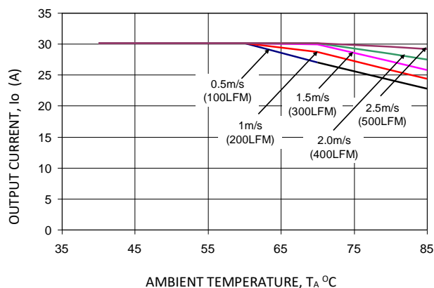
Figure 4. Derating Output Current versus Ambient Temperature and Airflow (ATS030A0X3-SRH).
