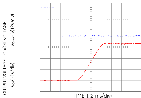
Figure 16. Typical Start-Up Using Remote On/Off with Low-ESR external capacitors (7x150μF Polymer) ( V_{in} = 5.0 Vdc, V_o = 3.3 Vdc, I_o = 5.0 A, C_o = 1050 μF).
