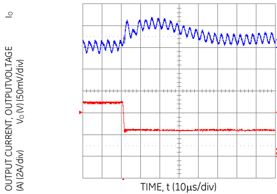
Figure 14. Transient Response to Dynamic Load Change from 100% of 50% full load ( V_o = 5.0 Vdc, C_{ext} = 2 \times 150 μF Polymer Capacitors).
