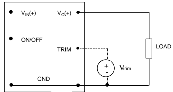
Figure 32. Circuit Configuration for programming Output voltage using external voltage source.
