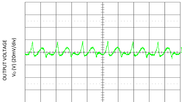
Figure 8. Typical Output Ripple and Noise ( V_{in} = 12.0V dc, V_o = 2.5 Vdc, I_o=10A ).
