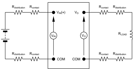
Figure 24. Output Ripple and Noise Test Setup.
