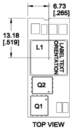
Figure 33. Pick and Place Location.
