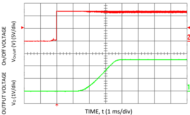
Figure 15. Typical Start-Up Using Remote On/Off with Low-ESR external capacitors (Co = 5000µF) (Vin = 12.0Vdc, Vo = 5.0Vdc, Io = 10.0A, Co = 1050µF).
