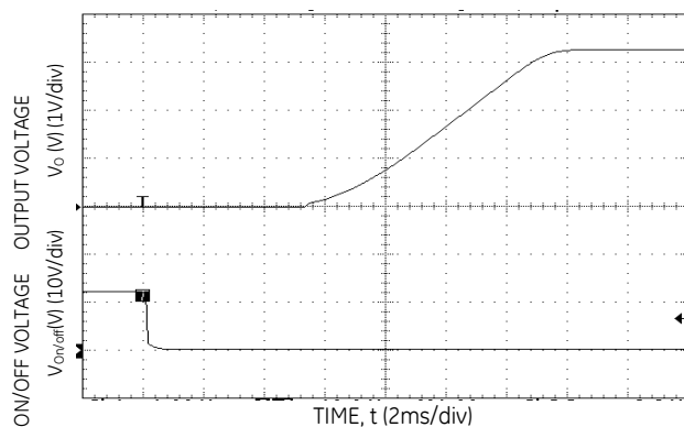
Figure 15. Typical Start-Up Using Remote On/Off with Low-ESR external capacitors (7x150µF Polymer) ( V_{IN} = 12.0\text{Vdc} , V_o = 3.3\text{Vdc} , I_o = 3\text{A} , C_o = 1050\text{ }\mu\text{F} ).
