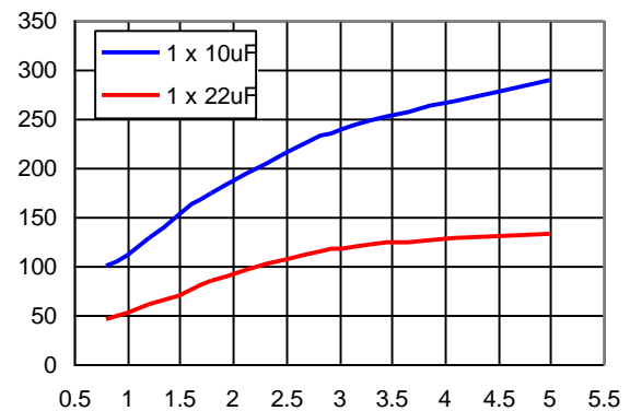
Figure 26. Input ripple voltage for various outputs with a 10 μF or a 22 μF ceramic capacitor at the input (full-load).
