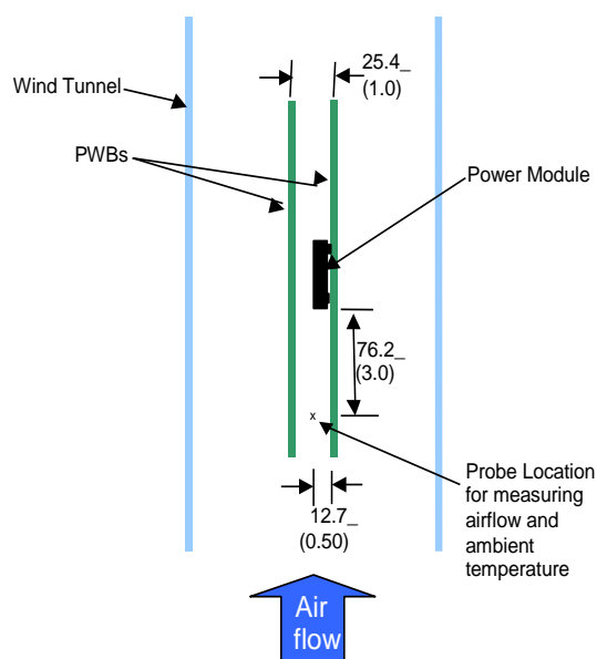
Figure 33. Thermal Test Up
