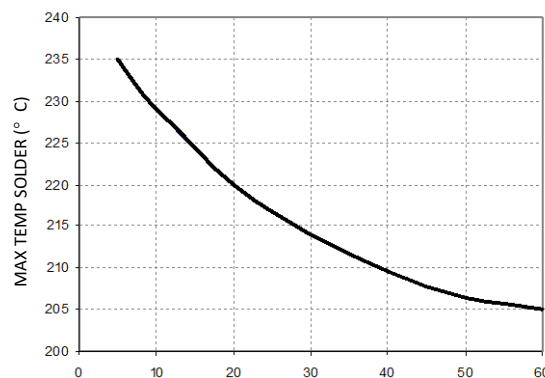
Figure 38. Time Limit Curve Above 205°C Reflow for Tin Lead (Sn/Pb) process.
