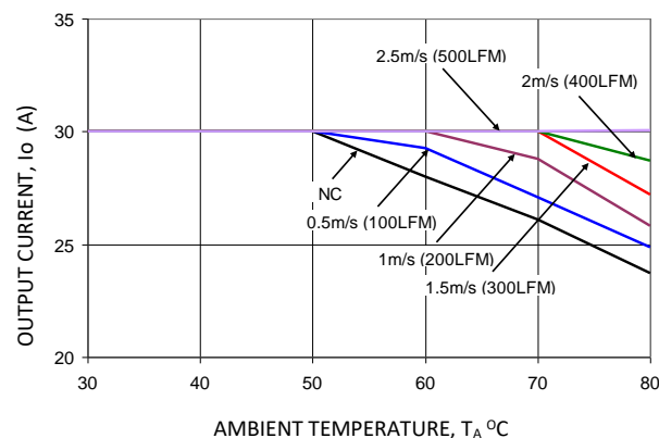
Figure 11. Derating Output Current versus Ambient Temperature and Airflow (ATM030A0X3-SRH).
