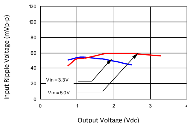
Figure 27. Input ripple voltage for various output with 2x150 μF polymer and 2x47 μF ceramic capacitors at the input (80% of I_{O,max} ).
