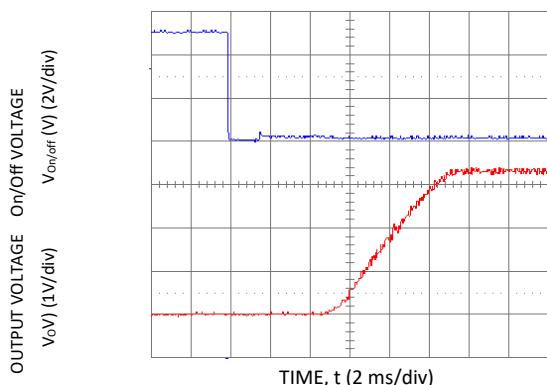
Figure 15. Typical Start-Up Using Remote On/Off with Low-ESR external capacitors (7x150uF Polymer) ( V_{in} = 5.0\text{Vdc} , V_o = 3.3\text{Vdc} , I_o = 6\text{A} , C_o = 1050\mu\text{F} ).
