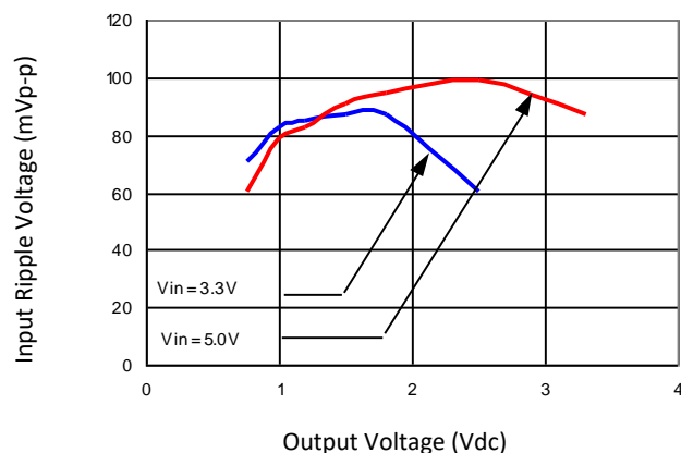
Figure 26. Input ripple voltage for various output with 1x150 μF polymer and 1x47 μF ceramic capacitors at the input (80% of I_{O,max} ).
