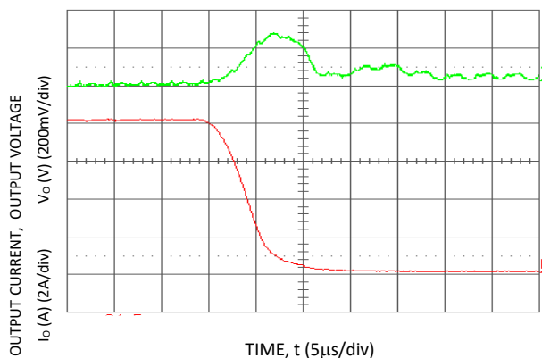
Figure 11. Transient Response to Dynamic Load Change from 100% to 50% of full load ( V_O = 3.3\text{Vdc} ).
