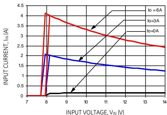
Figure 7. Input voltage vs. Input Current ( V_{out} = 5Vdc ).
