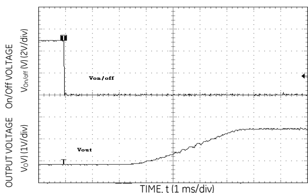
Figure 15. Typical Start-Up Using Remote On/Off with Low-ESR external capacitors (7x150uF Polymer) ( V_{in} = 12 Vdc, V_o = 3.3 Vdc, I_o = 6.0 A, C_o = 1050 \mu F).
