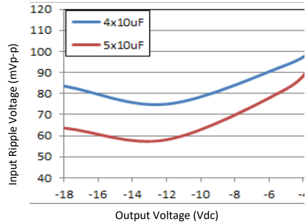
Figure 66. Input ripple voltage with 4x10 µF or 5x10 µF input ceramic capacitors (max load).
