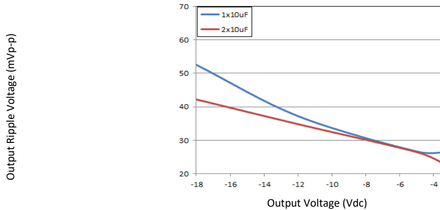
Figure 68. Output ripple with 1x10 \mu F or 2x10 \mu F output ceramic capacitors (max load).
