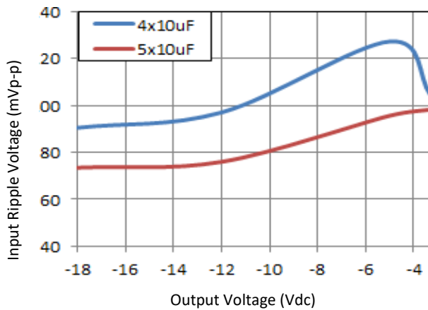
Figure 64. Input ripple voltage with 4x10 µF or 5x10 µF ceramic capacitors at the input (max load).
