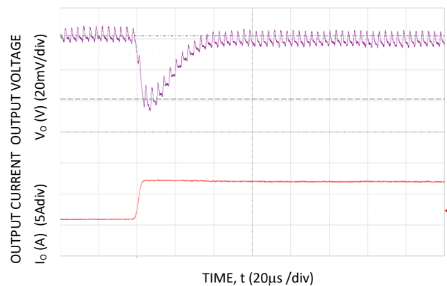
Figure 4. Transient Response to Dynamic Load Change from 50% to 100% at 28Vin, Cext – 2x22μF+2x330μF, CTune=15nF & RTune=200Ω
