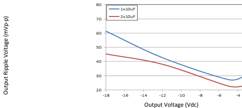
Figure 69. Output ripple with 1x10 \mu F or 2x10 \mu F output ceramic capacitors (max load).
