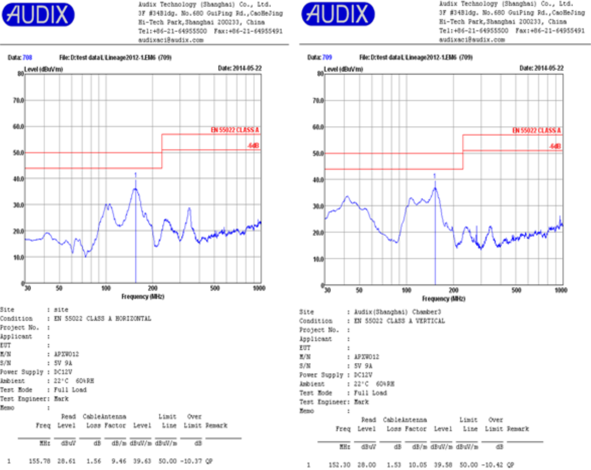
Fig 43 – EMI Plot of APXW012 on evaluation board with 12 V in, 5Vo @ 9 A out
