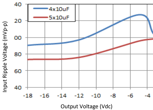
Figure 64. Input ripple voltage with 4x10 µF or 5x10 µF ceramic capacitors at the input (max load).
