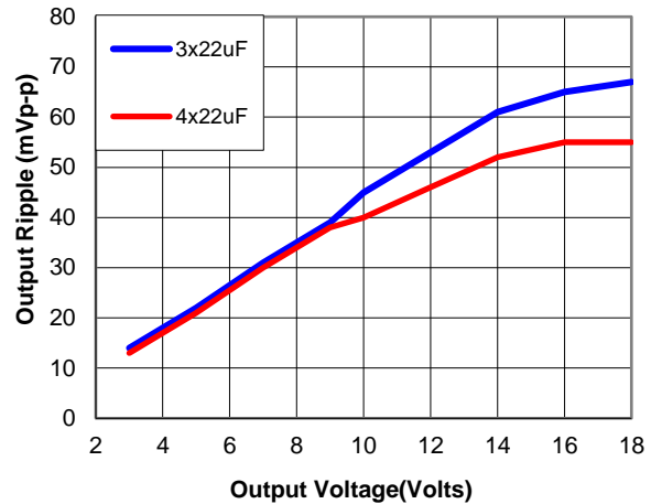
Figure 31. Output ripple voltage with external 3x22 \mu F or 4x22 \mu F ceramic capacitors at the output (max. load). Input voltage is 28V. Scope BW 20MHz
