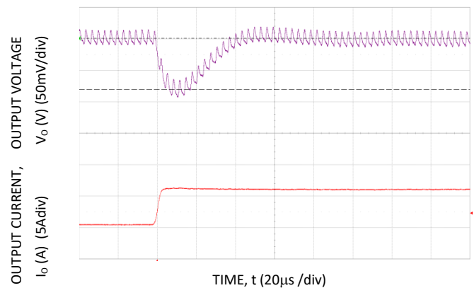
Figure 10. Transient Response to Dynamic Load Change from 50% to 100% at 28Vin, Cext – 1X22μF+1x330μF, CTune=5.6nF & RTune=200
