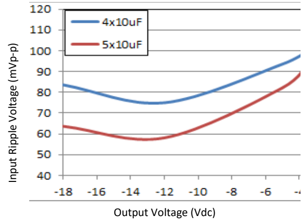
Figure 66. Input ripple voltage with 4x10 µF or 5x10 µF input ceramic capacitors (max load).
