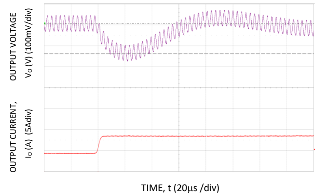
Figure 16. Transient Response to Dynamic Load Change from 50% to 100% at 28Vin, C_{ext} = 1 \times 22\mu F + 1 \times 470\mu F , C_{Tune} = 1.5nF & R_{Tune} = 200
