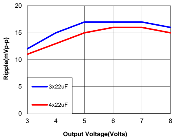
Figure 30. Output ripple with external 3x22 \mu F or 4x22 \mu F ceramic capacitors at the output (max. load). Input voltage is 12V. Scope BW at 20MHz
