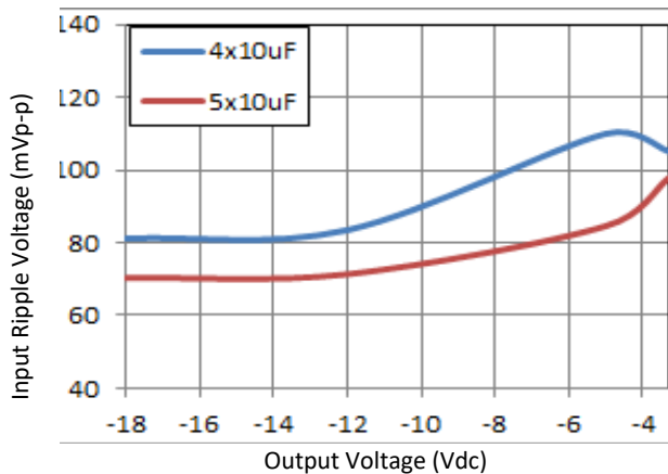
Figure 65. Input ripple voltage with 4x10 µF or 5x10 µF ceramic capacitors at the input (max load).
