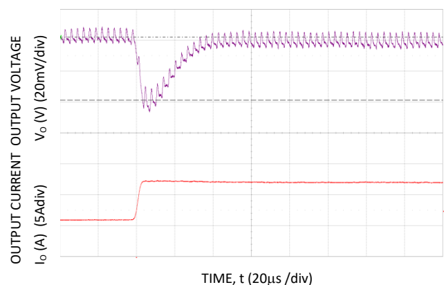
Figure 4. Transient Response to Dynamic Load Change from 50% to 100% at 28Vin, C_{ext} = 2 \times 22\mu F + 2 \times 330\mu F , C_{Tune} = 15nF & R_{Tune} = 200\Omega
