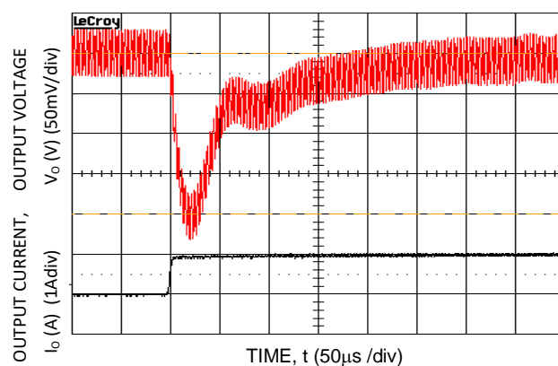
Figure 16. Transient Response to Dynamic Load Change from 50% to 100% at 28V in , C ext - 3x10uF ceramic, C Tune =47pF & R Tune =332Ω
