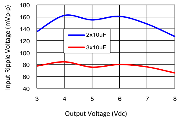
Figure 28. Input ripple voltage for various output voltages with 2x10 μF or 3x10 μF ceramic capacitors at the input (maximum load). Input voltage is 12V
