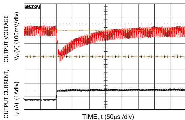
Figure 22. Transient Response to Dynamic Load Change from 50% to 100% at 28V in , C ext - 1x10μF ceramic, C Tune =open & R Tune =open
